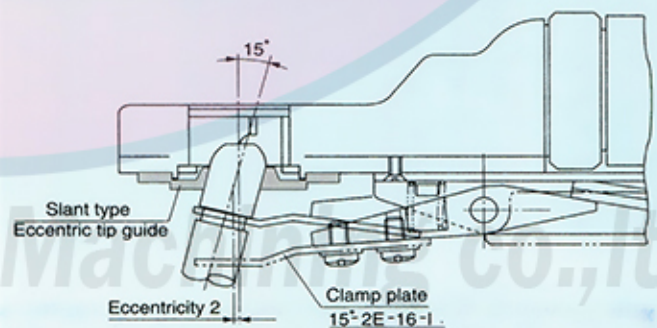
Tool type ETD-25A-E
